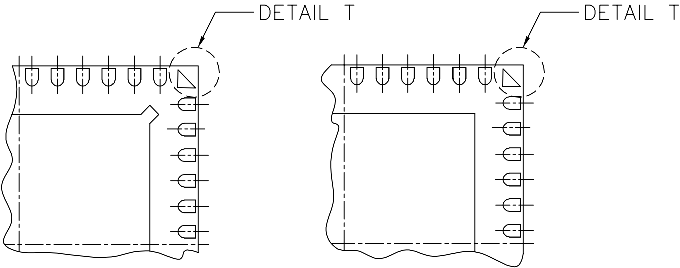
DETAIL M PIN 1 BACKSIDE IDENTIFIER OPTION
