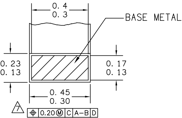
SECTION B-B VIEW ROTATED 90°
