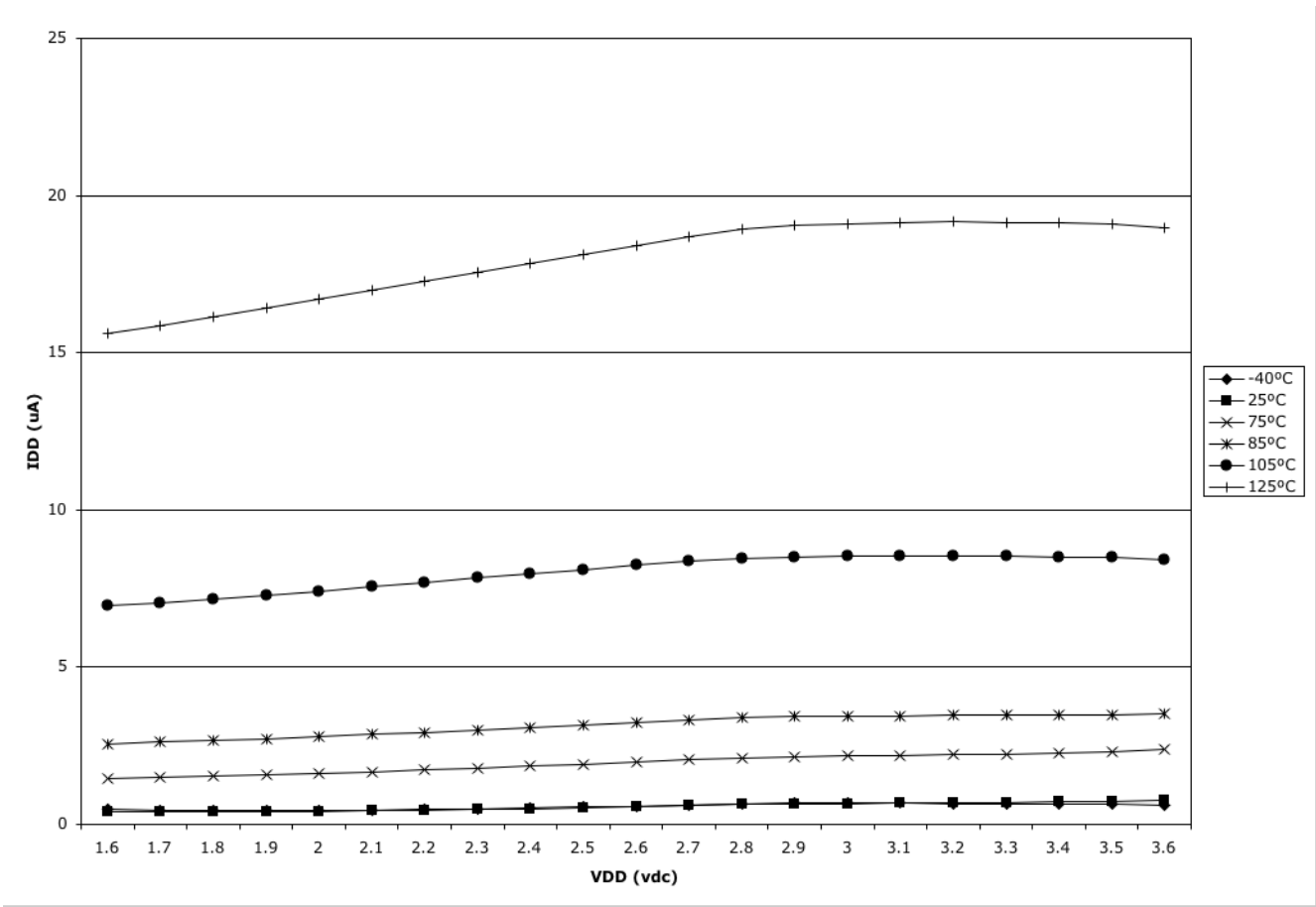
Figure A-9. Typical Stop3 I_{DD}
