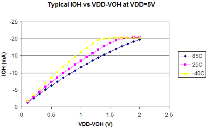
Figure 12-8. Typical IOH vs. VDD-VOH VDD = 5 V
