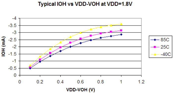
Figure 12-10. Typical IOH vs. VDD-VOH VDD = 1.8 V
