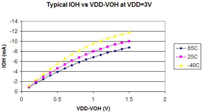
Figure 12-9. Typical IOH vs. VDD-VOH VDD = 3 V
