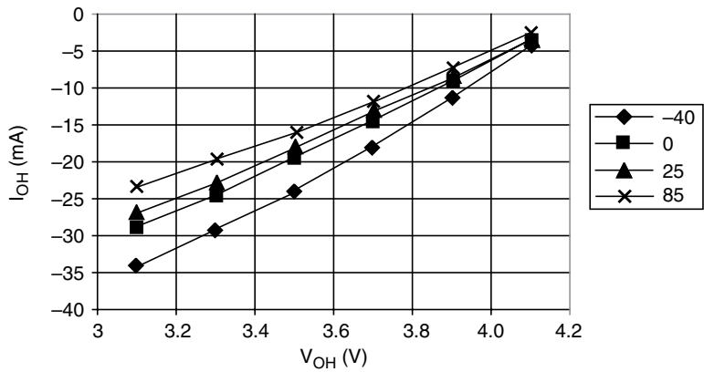
Figure 19-4. Typical High-Side Driver Characteristics – Port PTC4–PTC0 ( V_{DD} = 4.5 \text{ Vdc} )
