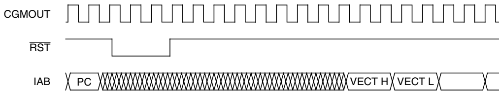
Figure 14-4. External Reset Timing
