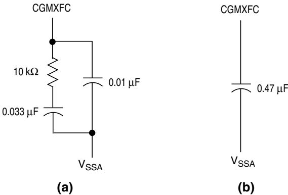
Figure 5-10. PLL Filter
