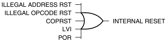
Figure 14-6. Sources of Internal Reset
