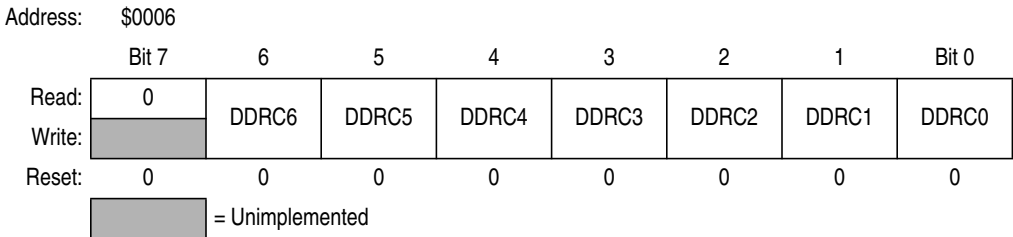
Figure 12-10. Data Direction Register C (DDRC)
