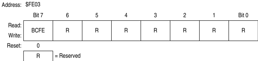
Figure 18-7. SIM Break Flag Control Register (SBFCR)
