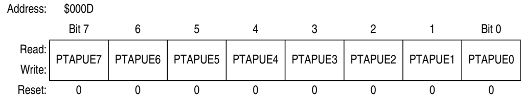
Figure 12-5. Port A Input Pullup Enable Register (PTAPUE)
