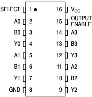
Figure 1. Pin Assignment
