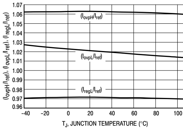
Figure 13. (I_{\text{OVPH}}/I_{\text{REF}}) , (I_{\text{OVL}}/I_{\text{REF}}) , (I_{\text{REGL}}/I_{\text{REF}}) versus Temperature
