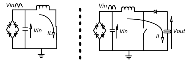
Figure 33. Off-Time Duration Increase
