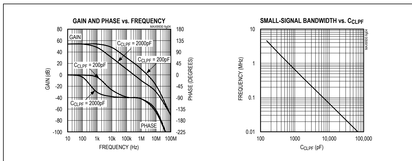
Figure 4. Gain and Phase vs. Frequency
