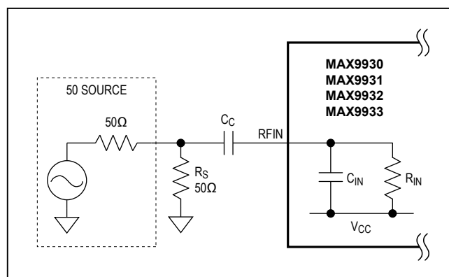
Figure 5. Broadband Resistive Matching
