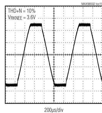
CLIPPING RESPONSE
