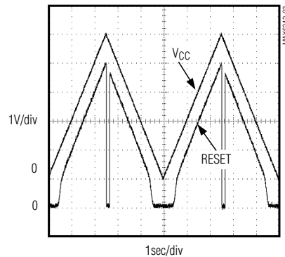
MAX6344L/MAX6345L RESET OUTPUT VOLTAGE vs. SUPPLY VOLTAGE
