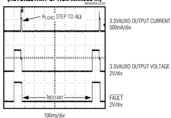
FAULT CONDITION ON AUXILIARY OUTPUT (AUTORESTART OPTION MAX5954A)
