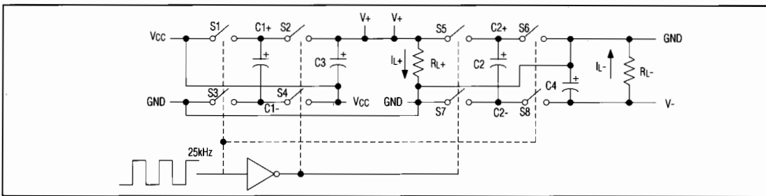
Figure 3. Charge Pump
