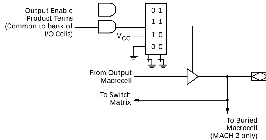
Figure 7. I/O Cell
