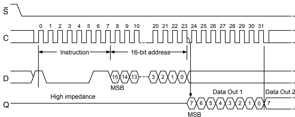
Figure 17. Read Lock status sequence
