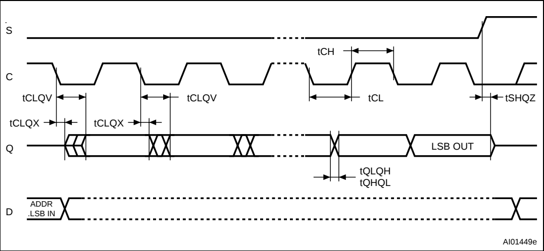
Figure 25. Output timing
