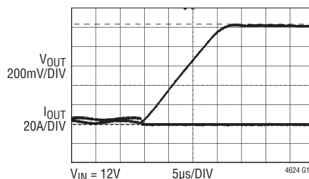
Recovery to No Load from Short Circuit
