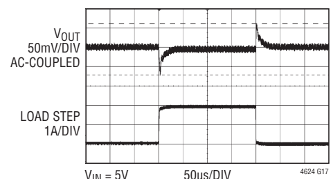
5V Input to 1.2V Output, 50% Load Transient Response
