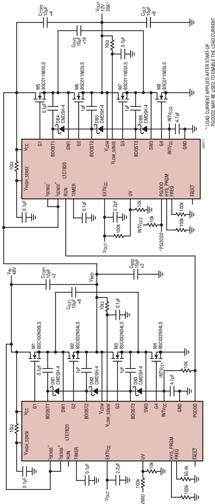
Figure 11. High Efficiency 48V to 12V, 20A Voltage Divider
