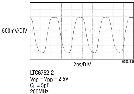
Output Toggle Waveform, LTC6752-2
