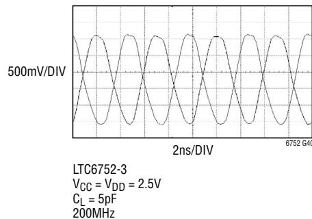
Output Toggle Waveforms Q and Q, LTC6752-3
