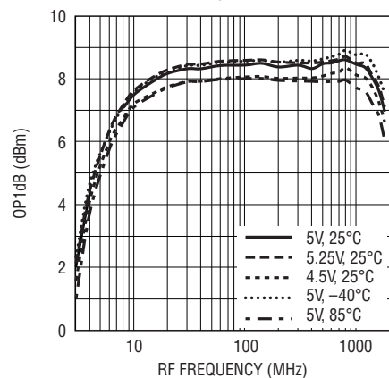
Output 1dB Compression vs RF Frequency
