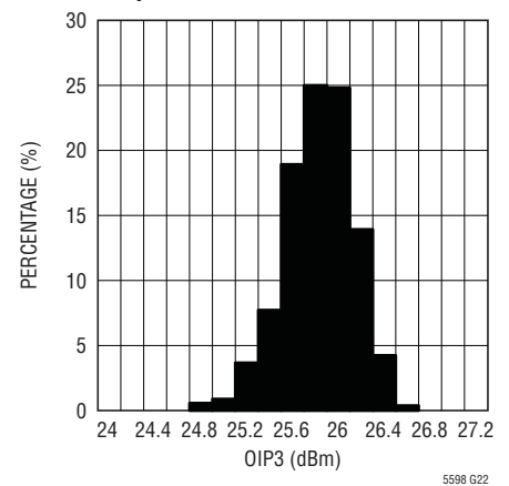
Output IP3 Distribution at 25°C
