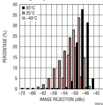
Image Rejection Distribution
