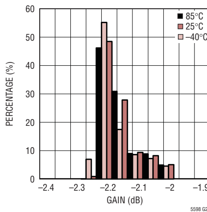
Gain Distribution
