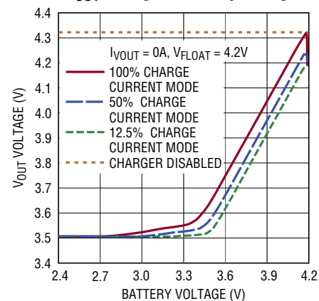
V_{OUT} Voltage vs Battery Voltage
