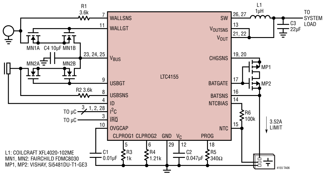
Dual-Input Overvoltage Protection with 1.21A Default Input Current Limit and Output Voltage Disconnect
