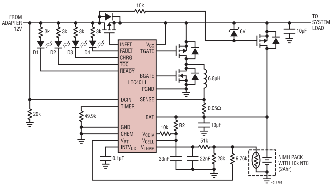
Figure 8. Full-Featured 2A LTC4011 Application
