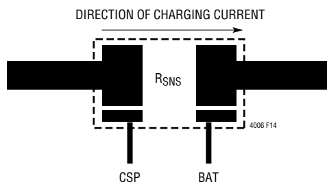
Figure 14. Kelvin Sensing of Charging Current
