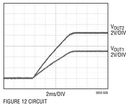
Soft Start-Up
