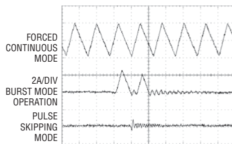
Inductor Current at Light Load
