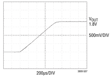
Start-Up with Internal Soft-Start
