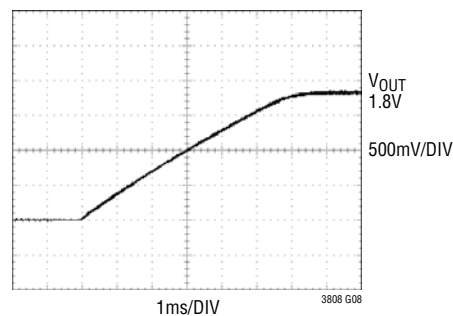
Start-Up with External Soft-Start ( C_{SS} = 10\text{nF} )
