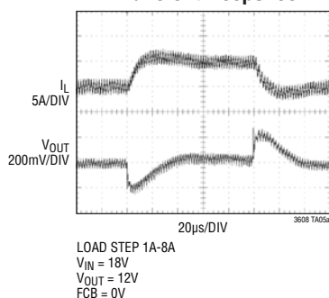
Transient Response
