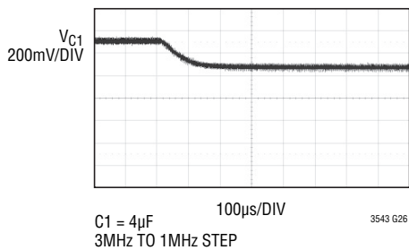
PLL Operation
