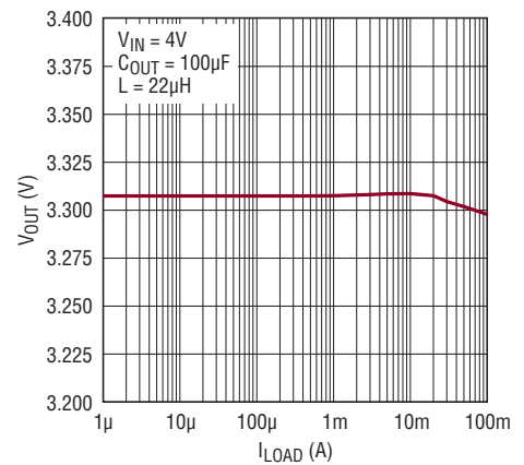
Buck Load Regulation, 3.3V
