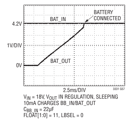
Battery Connect Transient
