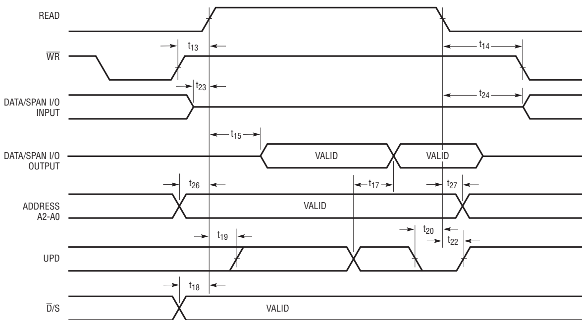
Readback Timing
