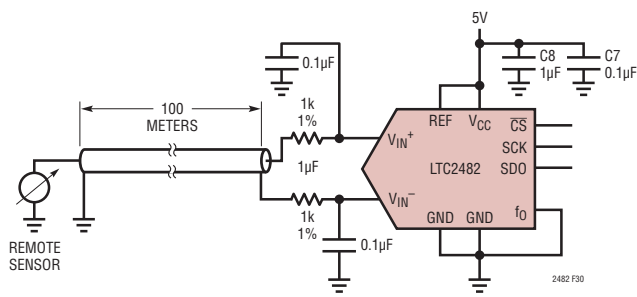
Figure 30. Differential Input Current Cancellation Enables Direct Digitization of Remote Sensors
