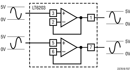
Figure 7. LT6203 Buffering a Fully Differential Signal Source
