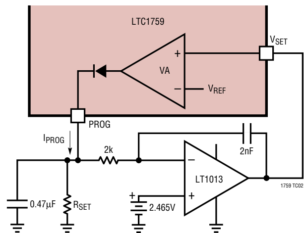
Test Circuit 2
