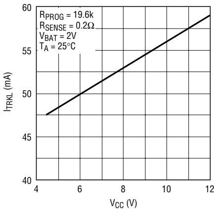
Trickle Charge Current vs Input Supply
