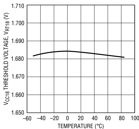
V CC18 Threshold Voltage vs Temperature (LTC1728-1.8/LTC1728-3.3)
