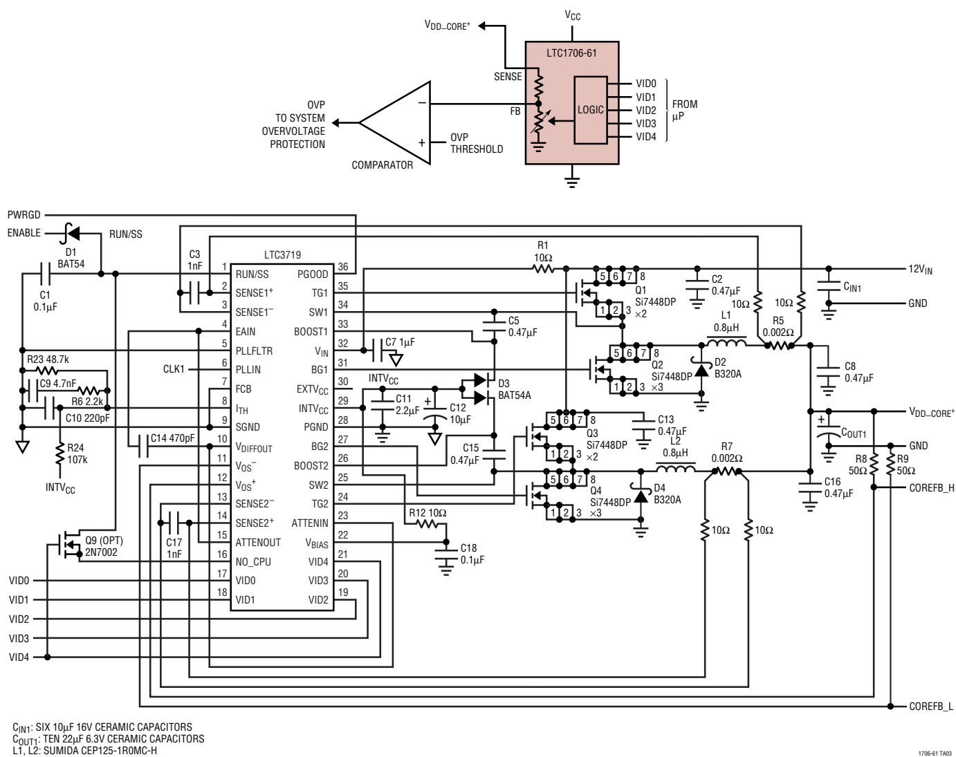
2-Phase 12V Input, 0.8V to 1.55V/45A Max Power Supply with Adjustable Overvoltage Protection
