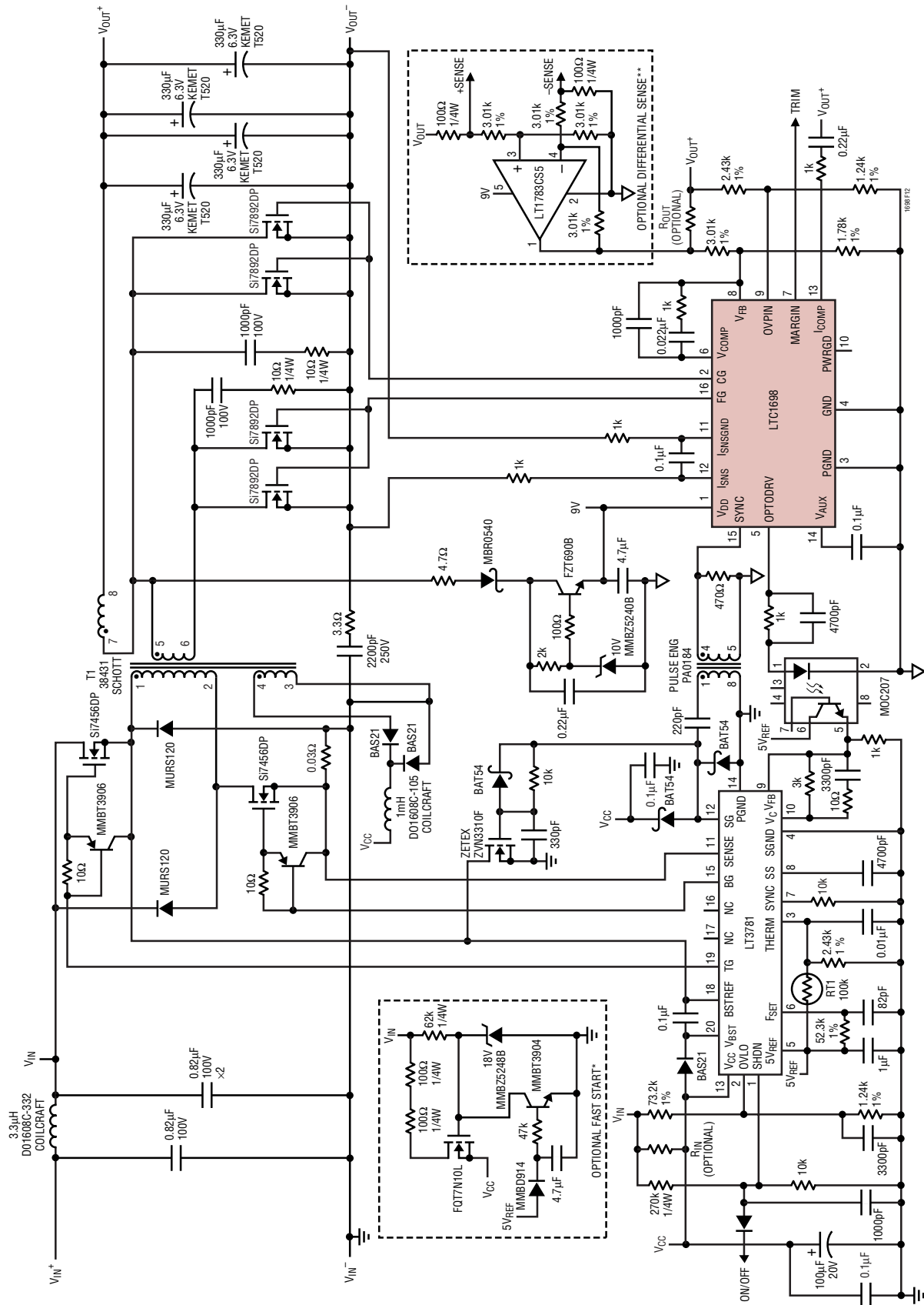
Figure 12. LT3781/LTC1698 36V IN -72V IN to 3.3V/15A Isolated Synchronous Forward Converter-Quarter Bridge
