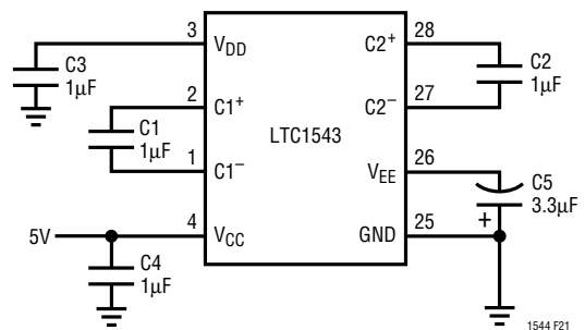
Figure 21. Charge Pump
