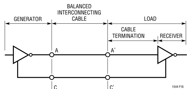
Figure 16. Typical V.28 Interface
