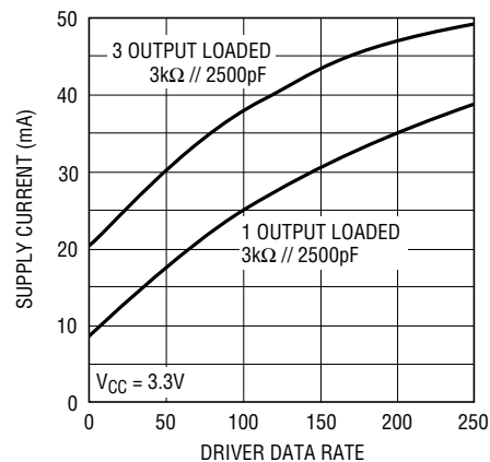
Supply Current vs Driver Data Rate
