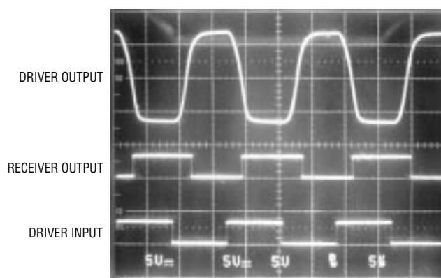
Figure 6. Driver Test Result at 120kbps
