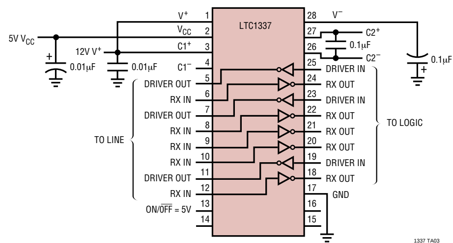
Operation Using 5V and 12V Power Supplies
