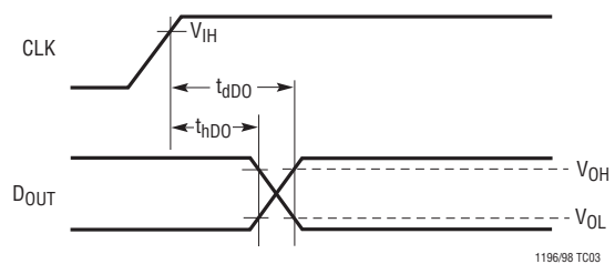
Voltage Waveform for D_{OUT} Delay Time, t_{dD0} , t_{hD0}
