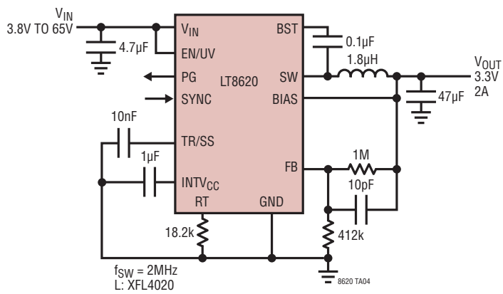
3.3V 2MHz Step-Down Converter
