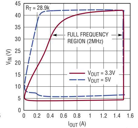
Channel 1 Full Frequency V_{IN} vs Load Current
