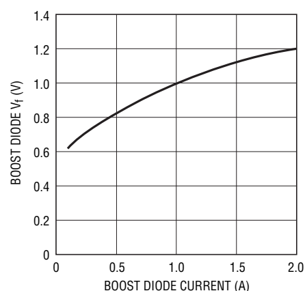
Boost Diode
