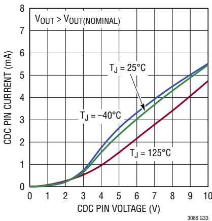
CDC Pin Internal Clamp Fault Current
