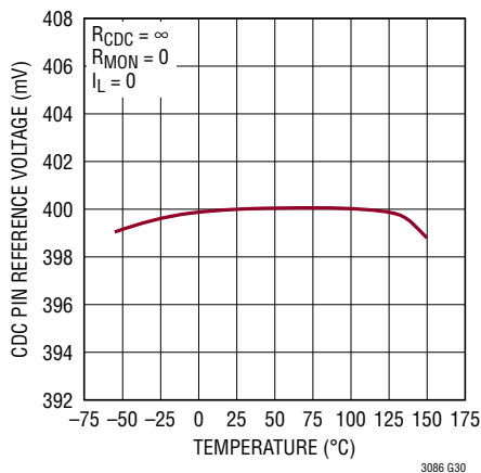
CDC Pin Reference Voltage
