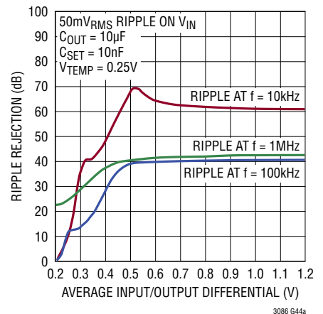
5V, 1A Ripple Rejection vs V_{IN} - V_{OUT}
