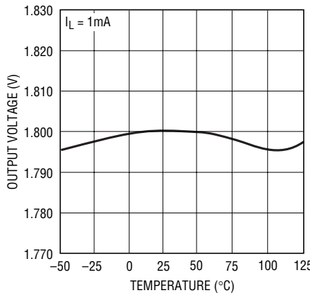
Output Voltage
