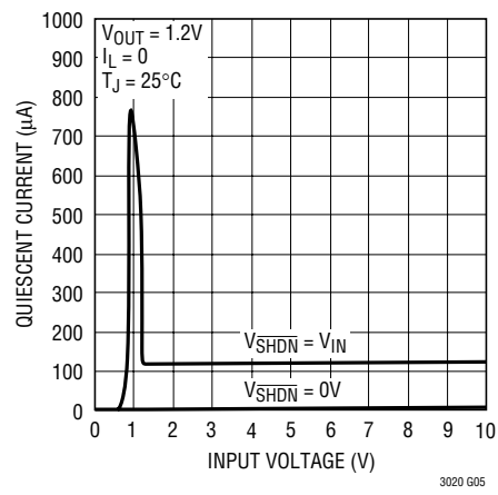
Quiescent Current
