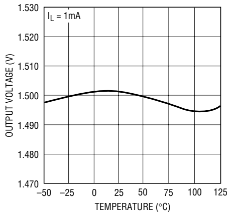
Output Voltage
