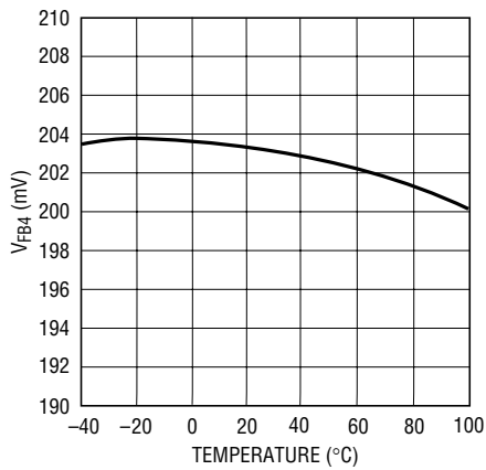
FB4 Voltage
