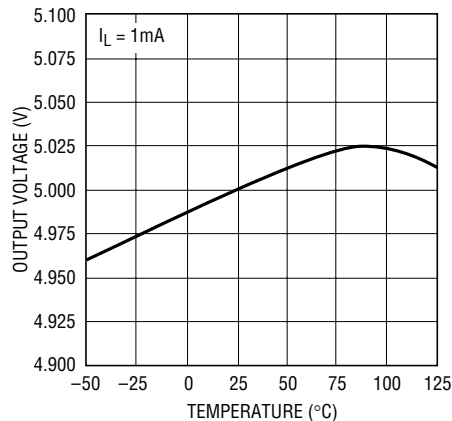
LT1762-5 Output Voltage
