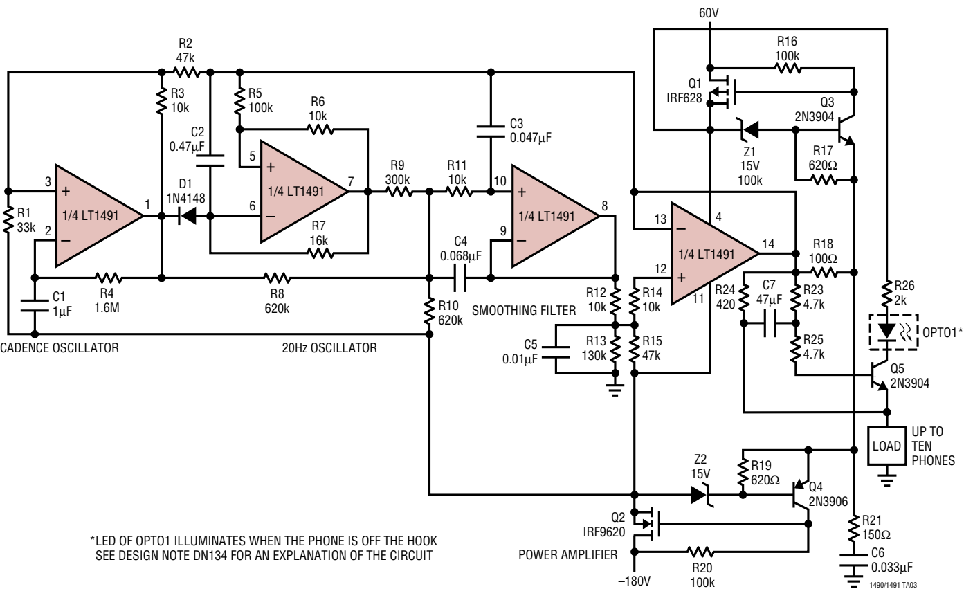
Ring-Tone Generator
