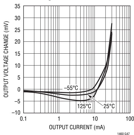
LT1460S3-10V Load Regulation, Sourcing
