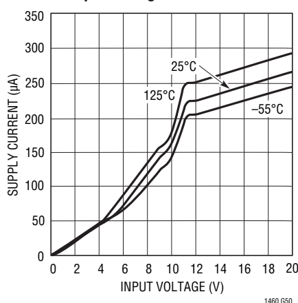
LT1460S3-10V Supply Current vs Input Voltage
