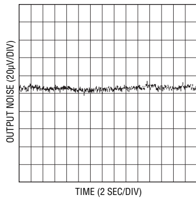
LT1460S3-2.5V Output Noise 0.1Hz to 10Hz
