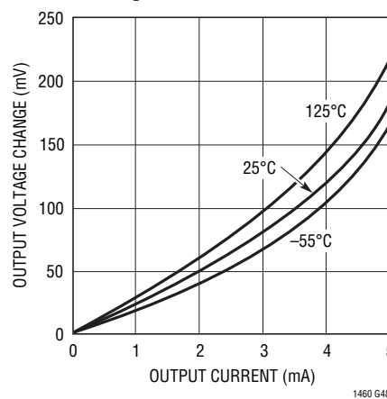
LT1460S3-10V Load Regulation, Sinking
