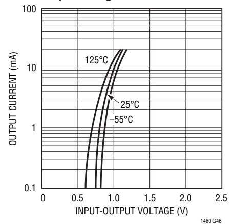
LT1460S3-10V Minimum Input-Output Voltage Differential
