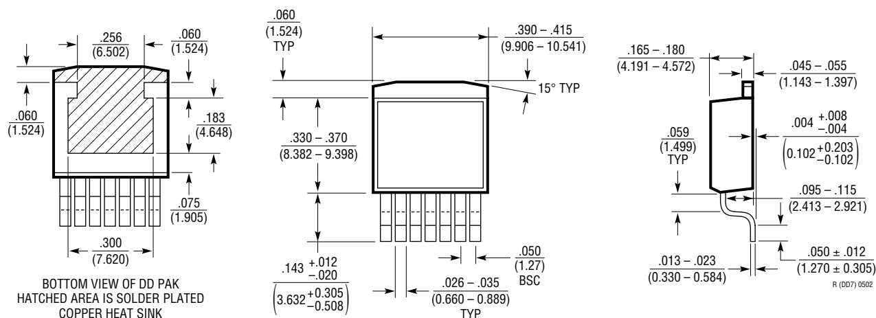
R Package 7-Lead Plastic DD Pak (LTC DWG # 05-08-1462)
